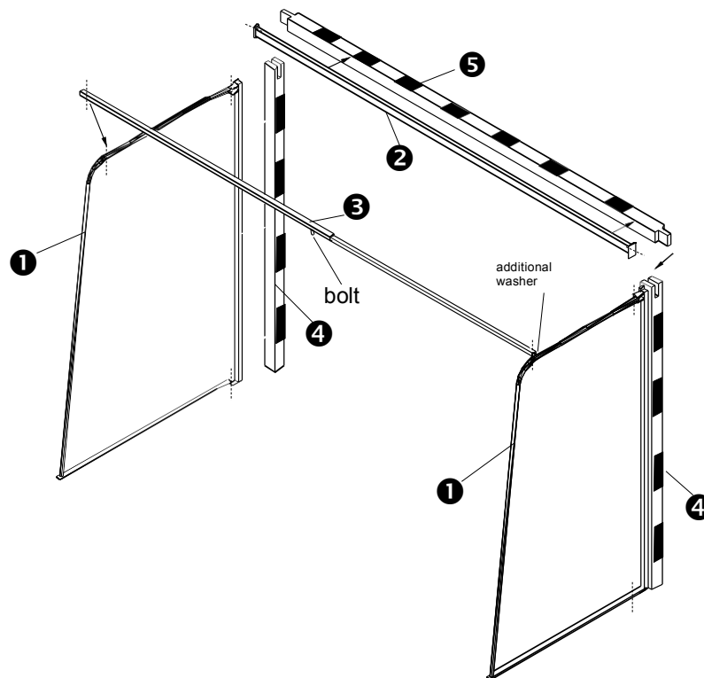
Ill. 2: Sport-Thieme 'Spezial' handball goal assembly drawing
